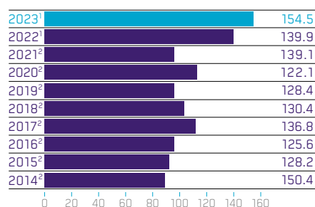
Capital ratio (%)
